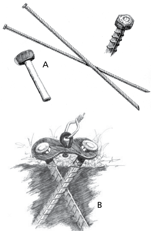
Figure 9. Metal stakes used to secure relaxing cable restraints into the earth. In poor substrate, it is recommended that two 30 inch (75cm) round metal stakes (e.g. re-rod; A) be hammered into the earth in a crosswise pattern (B).
