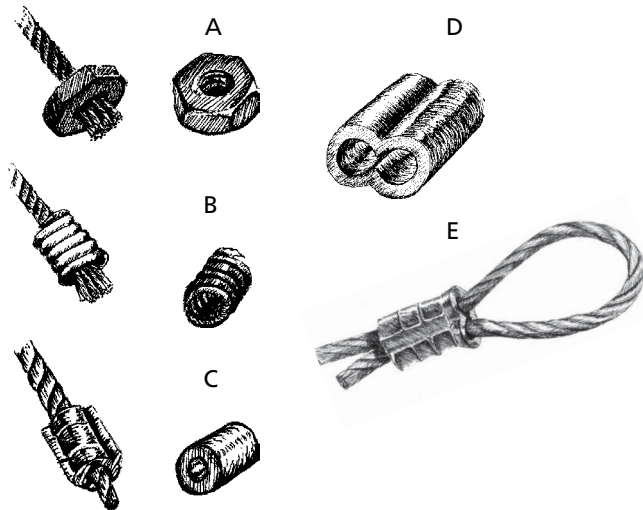
Figure 6. The diagram illustrates different types of cable stops, annealed steel nuts (A), coiled steel wire (B), aluminum ferrules (C), double end aluminum ferrules (D), and an end loop created with a double end ferrule (E) often used to attach the cable restraint to an anchor.
