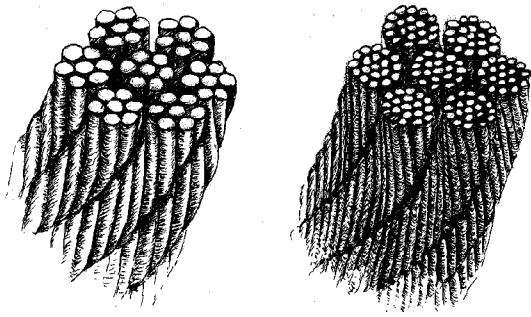
Figure 5. Illustration of a cross-section of a multi-strand cable used in cable restraint devices. Two commonly used patterns are a 7 by 7 design with 7 bundles of 7 wirestrands and a 7 by 19 design with 7 bundles of 19 wire strands.
